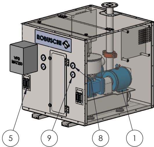
ISO VIEW
