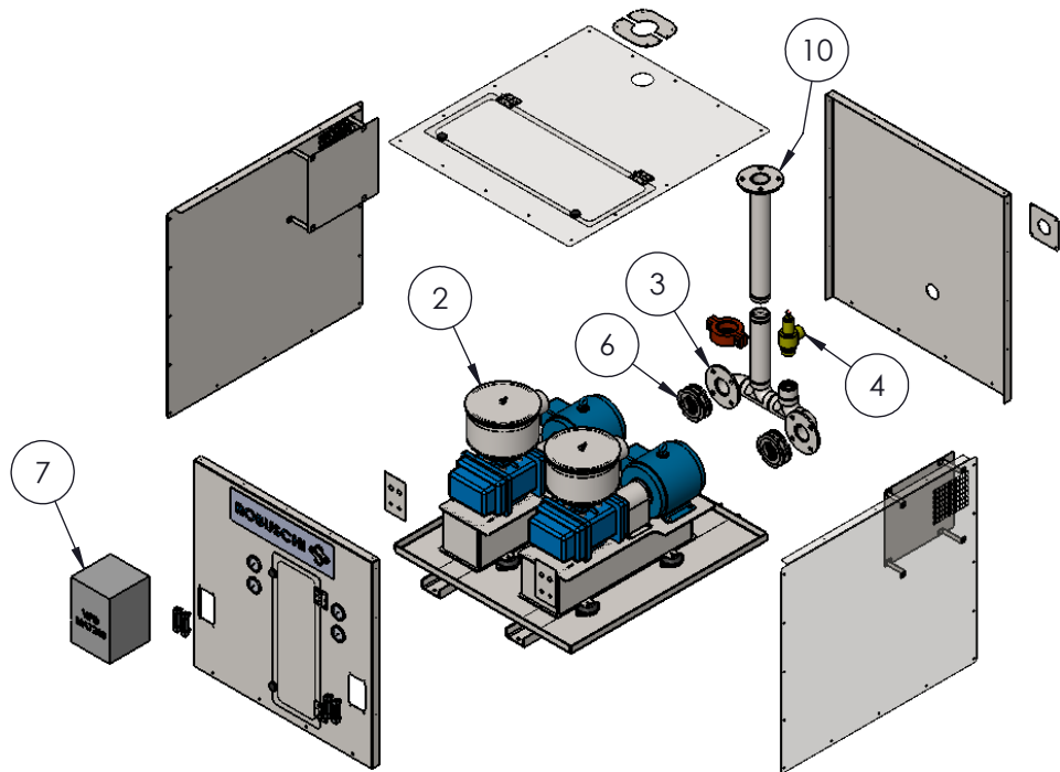
EXPLODED VIEW
